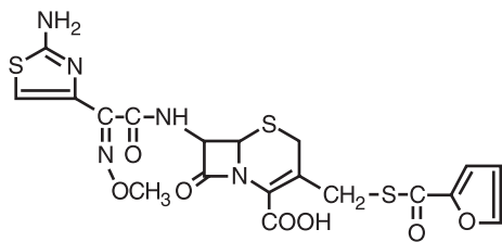
Figure 1. Structure of ceftiofur crystalline free acid:
